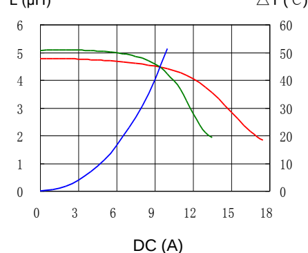
6. CDRH127L125NP-100MC
