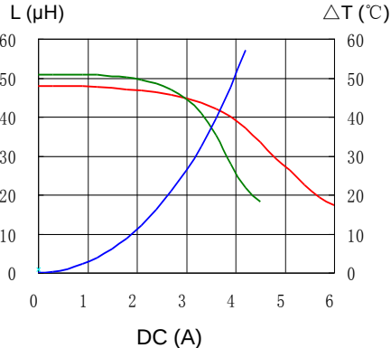
10. CDRH127L125NP-470MC
