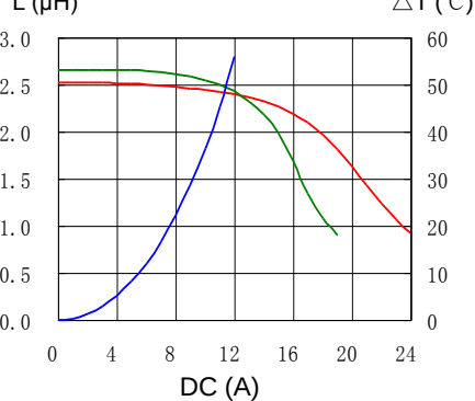
4. CDRH127L125NP-6R2NC
