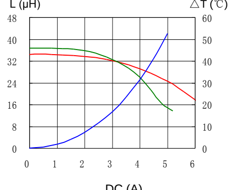
12. CDRH127L125NP-101MC
