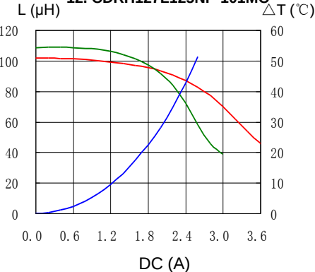
12. CDRH127L125NP-101MC
