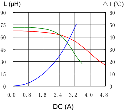
11. CDRH127L125NP-680MC
