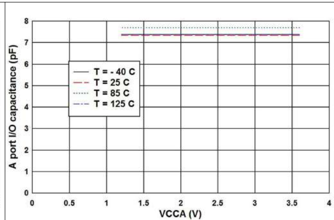
Figure 6-2. Capacitance for A port I/O pins ( C_{IO} ) vs Power Supply ( V_{CCA} ) for V_{CCB} = 3.3\text{ V} (RUT package)
