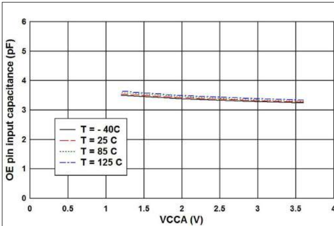
Figure 6-1. Input capacitance for OE pin ( C_I ) vs Power Supply ( V_{CCA} ) for V_{CCB} = 3.3\text{ V} (RUT package)
