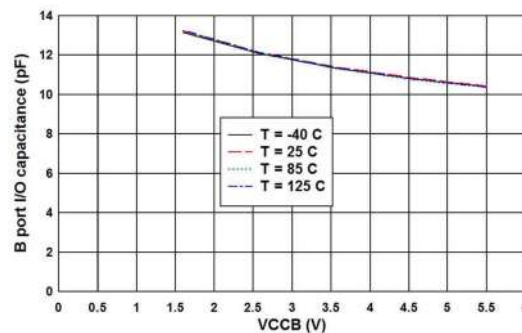
Figure 6-3. Capacitance for B port I/O pins ( C_{IO} ) vs Power Supply ( V_{CCB} ) for V_{CCA} = 3.3\text{ V} (RUT package)
