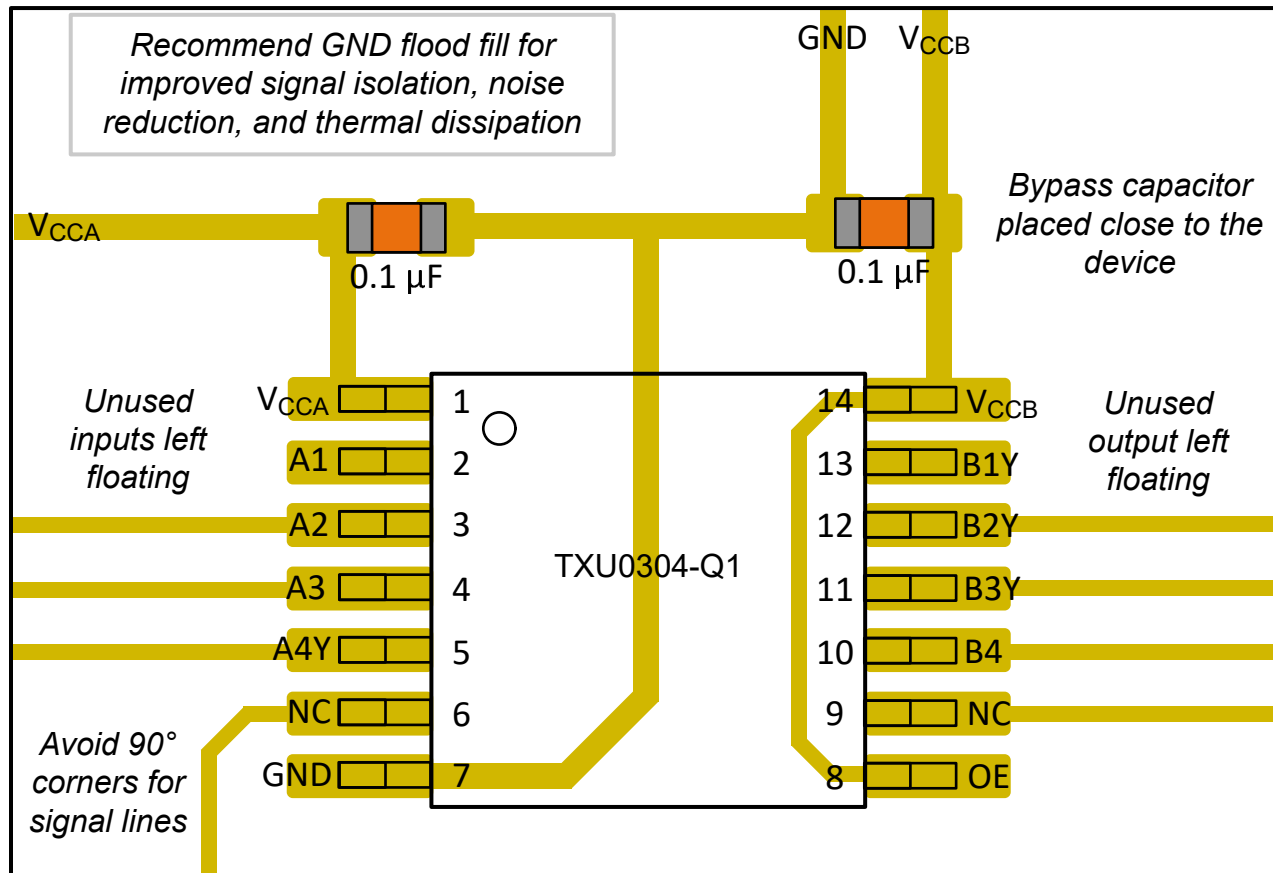
Figure 12-1. Layout Example – TXU0304-Q1
