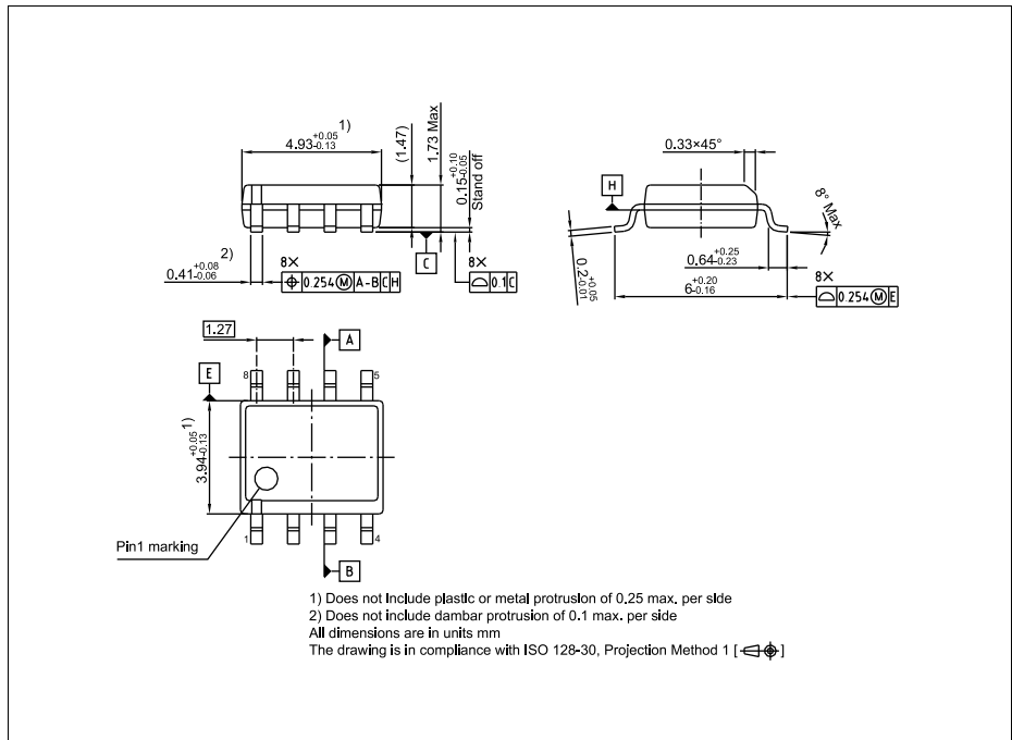
Figure 5 PG-DSO-8
