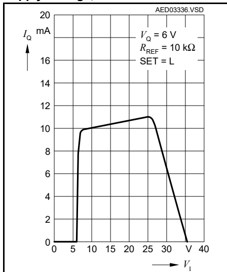
Output Current versus Supply Voltage, SET = L
