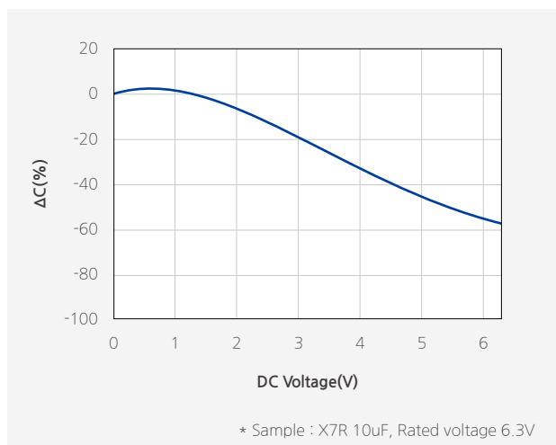
[ Example of DC Bias characteristics ]
